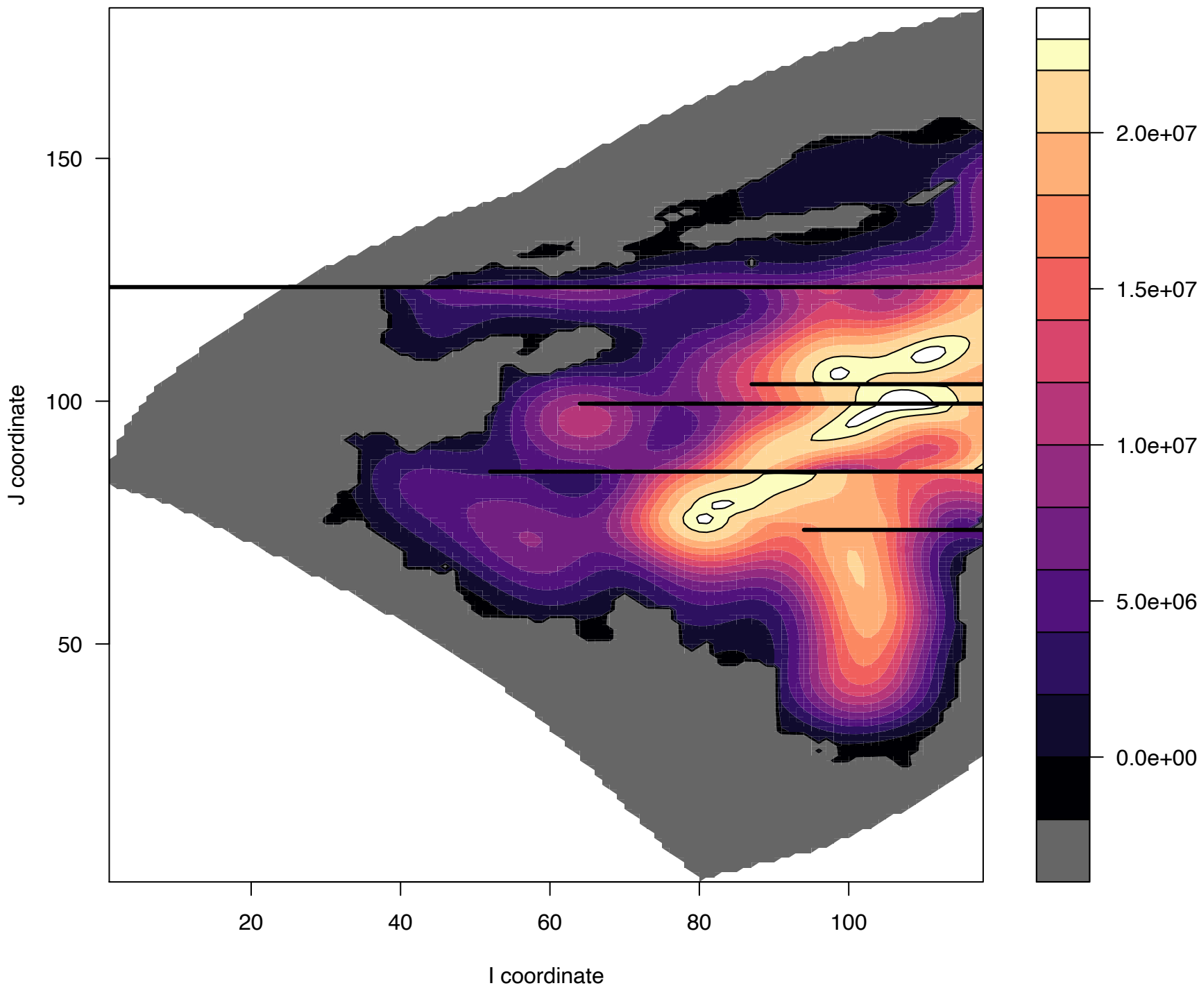
Plot of Emulator Expectation Well 1 Wave 2, Run = 95
